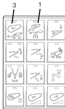
In-Cab Control Keypad
